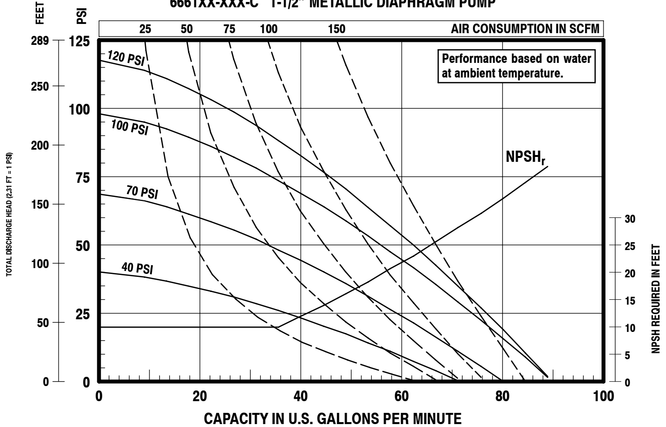
6661XX-XXX-C 1-1/2" METALLIC DIAPHRAGM PUMP
